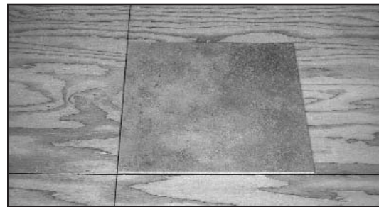
Fig. 9 - Positioning tiles.
