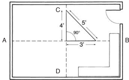
Fig. 6 - Square layout.
